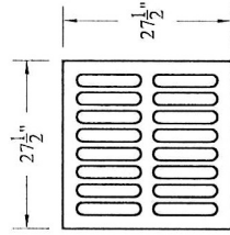
EJIW 5110 M-2 GRATE 1" THICK (144 LBS.)
