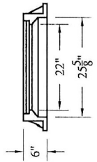
EJIW 5250 FRAME AND GRATE
