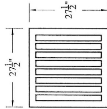
EJIW 5110 M-1 GRATE 1" THICK (120 LBS.)
