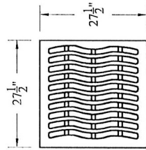
EJIW 5110 M-3 GRATE 1" THICK (165 LBS.)
