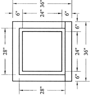
SLANT TOP PLAN VIEW
